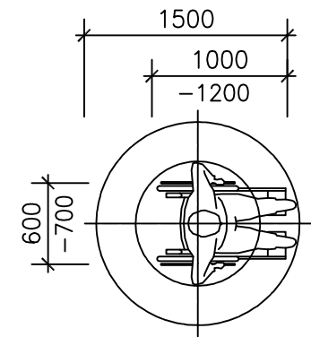
Floor space needed for manoeuvring a wheelchair.
